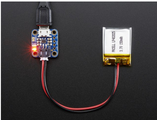
Adafruit Micro-Lipo Charger for LiPo/Lilon Batt w/MicroUSB Jack
