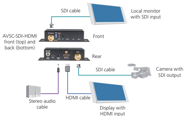
Figure 3-1. Typical application.
