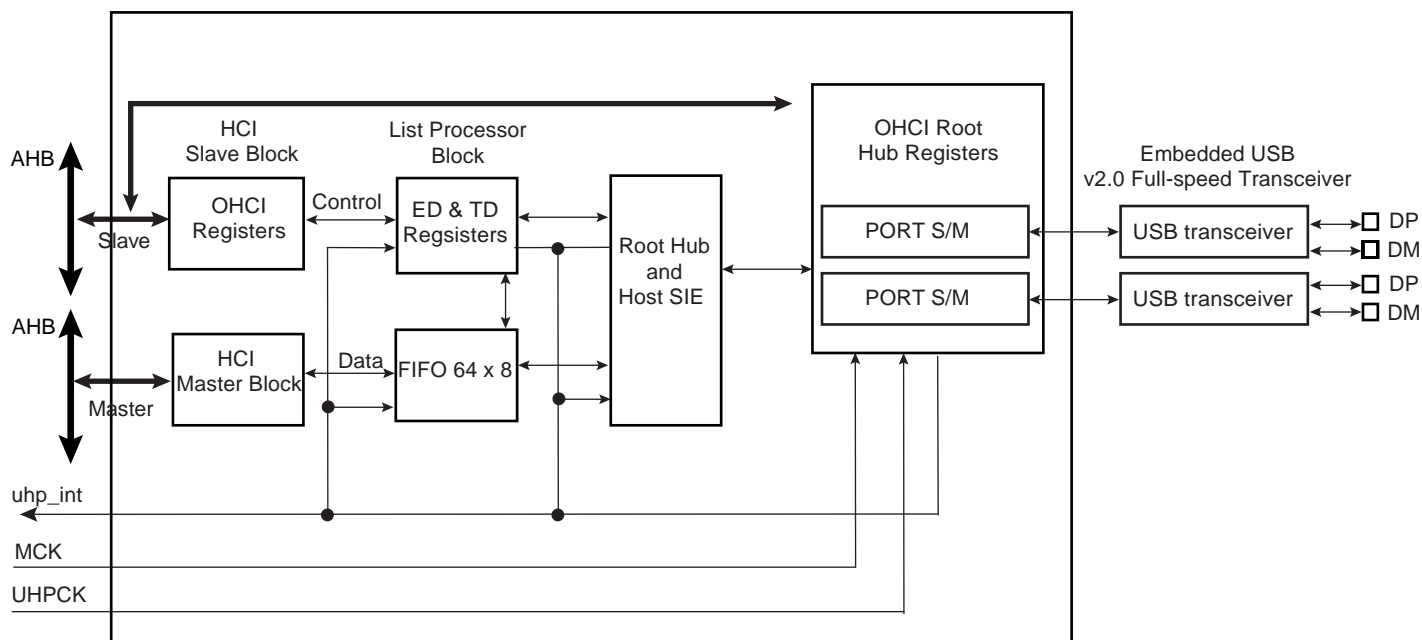
Figure 41-1. Block Diagram
