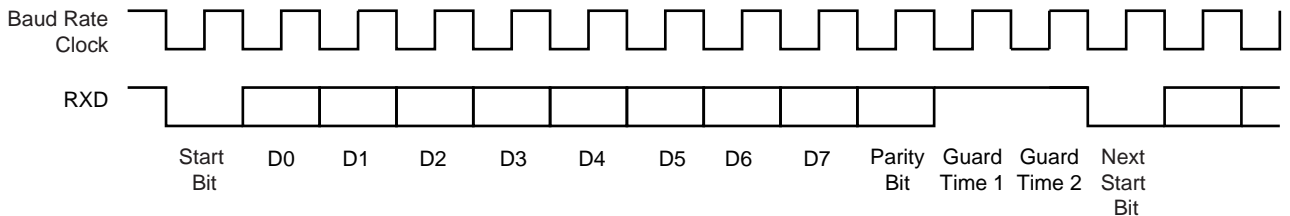
Figure 33-21. T = 0 Protocol without Parity Error
