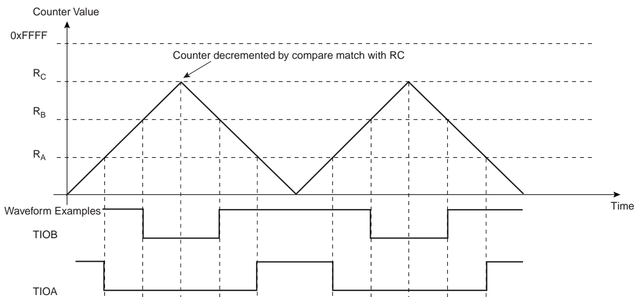
Figure 38-13. WAVSEL = 11 Without Trigger
