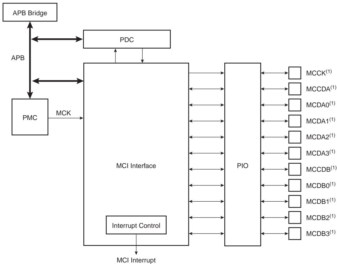
Figure 39-1. Block Diagram
