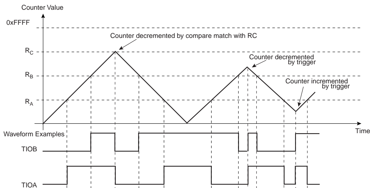
Figure 38-14. WAVSEL = 11 With Trigger
