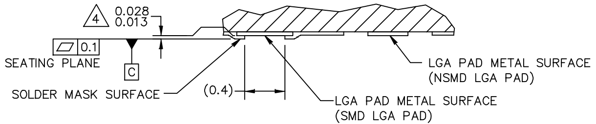
SECTION E-E 5
