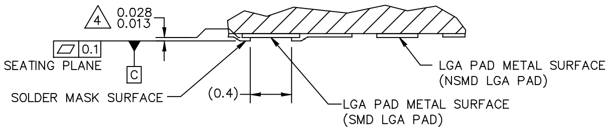
SECTION E-E 5
