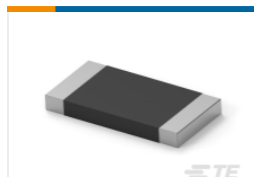
TE Part #5-2176422-6 TLRP 2512 3.0W R015 1% 50PPM 4K RL
