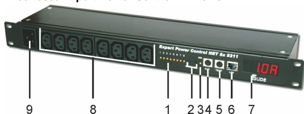
Anschlüsse Expert Power Control NET 8x 8211
