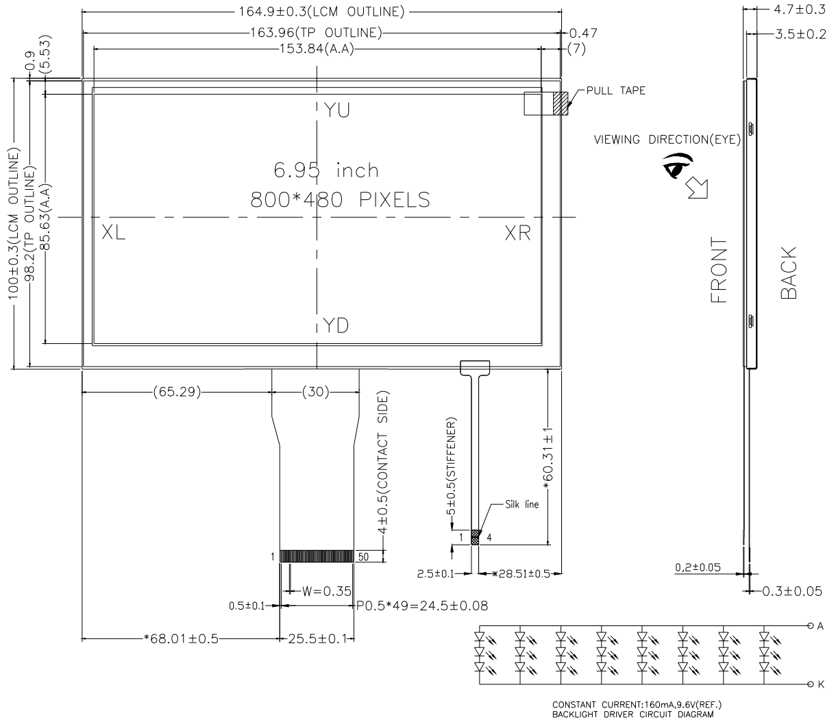
LCM(PIN DEFINE)
