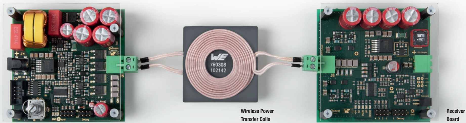
Transmitter Board
