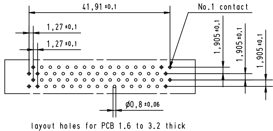
Printed Board Layout component side
