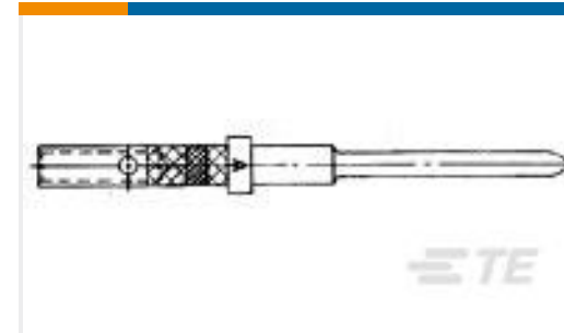
TE Part #204938-3 ARINC,PIN CONTACT,SZ 20
