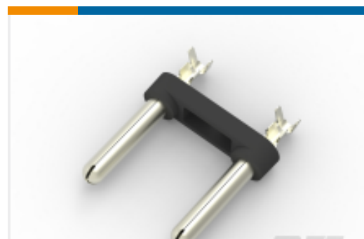
TE Part #2819037-1 WALL PLUG 2 POS. ASSY
