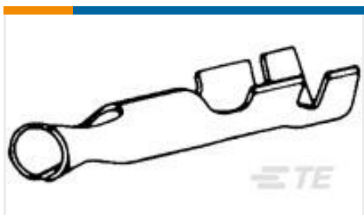
TE Part #42428-8 040 PIN REC IS 24-20 SPPHBZ
