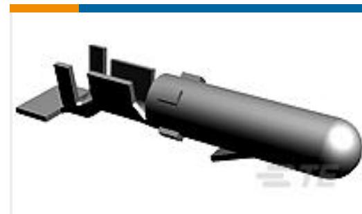
TE Part #61086-1 .156 MNL PIN 20-14 PTPBR
