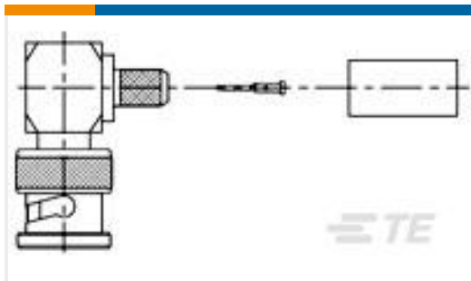
TE Part #1-1478075-0 BNC R/A Plg Hex 50Ohm Silver Pltd RG58C/
