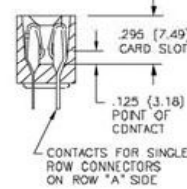
SECTION THROUGH CONTACT POSITION
