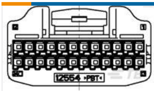
TE Part #1318917-1 025 ECU PLUG HSG ASSY 24P
