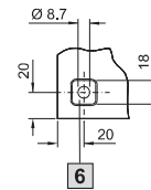
View A for wall mounting
