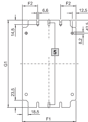
Mounting plate
