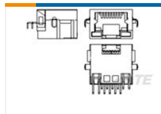
TE Part #2041411-1 RJ45 w/ LED, Tab Up, Offset, DIP, H=9.45
