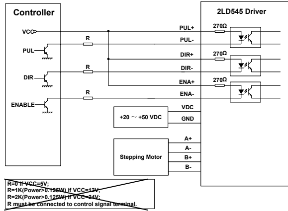
Figure 9: Typical connection
