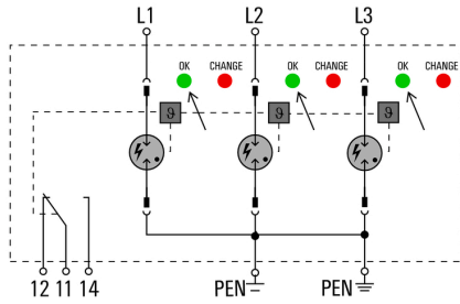
Schematic circuit diagram
