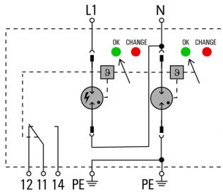
Schematic circuit diagram
