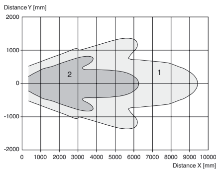
Distance Y [mm] 2000 1000 0 -1000 -2000 0 1000 2000 3000 4000 5000 6000 7000 8000 9000 10000 Distance X [mm] Curve 1: flat surface 100 mm x 100 mm Curve 2: round bar, Ø 25 mm
