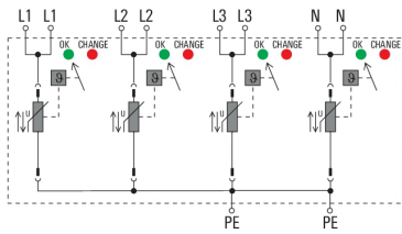
Schematic circuit diagram
