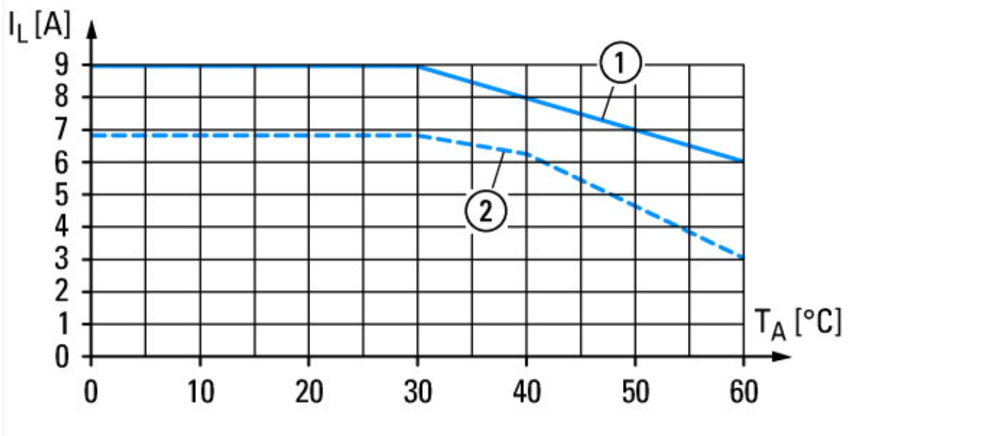
Electricity derating devices with I_o = 9 A ① For devices installed with a minimum clearance of 20 mm ② For devices in direct sequence
