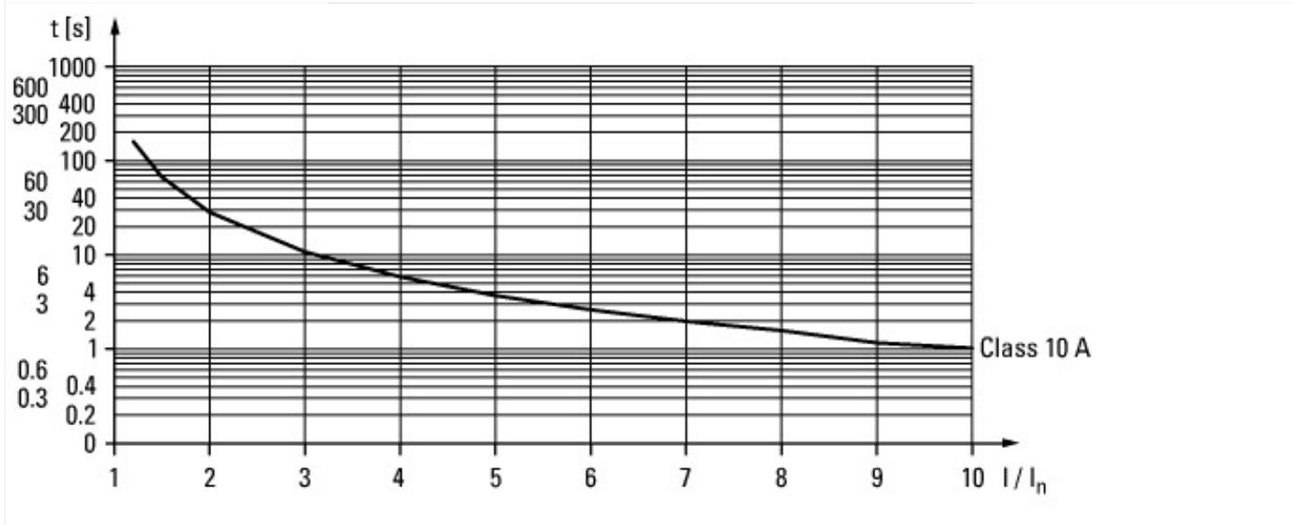
Tripping characteristic curve CLASS 10A set motor current > 4 A
