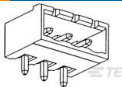
TE Part #796644-6 6POS 5.0MM CE R/A HDR,TRM BLK
