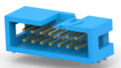
TE Part # 2-1761605-5 IDC LOW PRO HDR 14P RA BLUE
