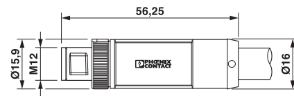
Dimensional drawing
