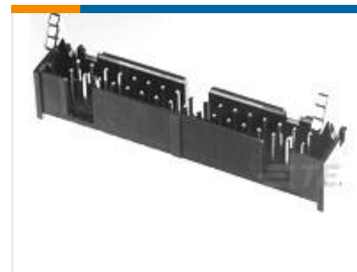
TE Part #2-1761606-9 IDC LOW PRO HDR 26P VERT LG LA
