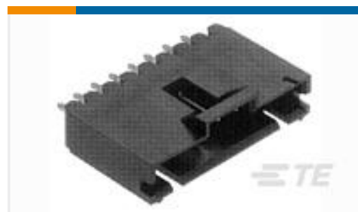
TE Part #103639-7 08 MTE HDR SRST LATCH .100CL
