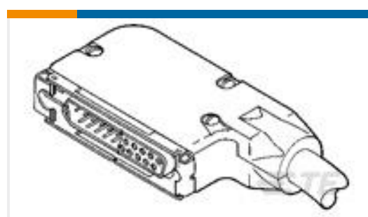
TE Part #5745653-4 DIECAST STRAIN RELIEF KIT, SZ 3
