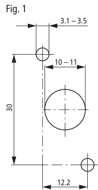
Fig. 1 Abmessungen – Dimensions [mm]
