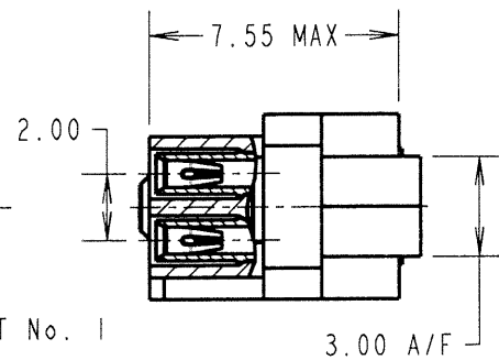
PART SECTION X-X
