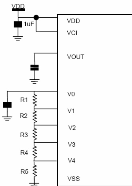
Figure 6-13: On-chip voltage converter application set up
