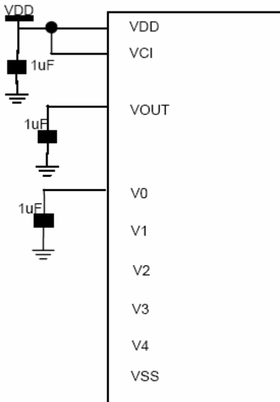
Figure 6-13: On-chip voltage converter application set up
