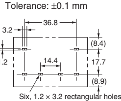
PCB Mounting Holes
