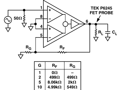
TPC 18. AD8130 Basic Frequency Response Test Circuit
