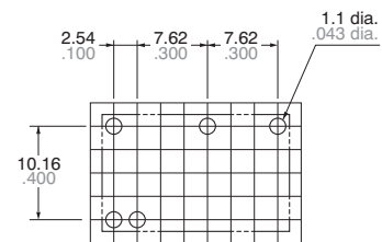
2 coil latching
