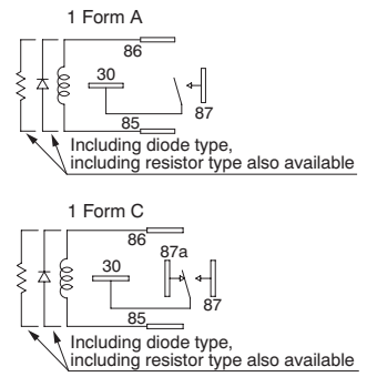
Schematic (Bottom view)
