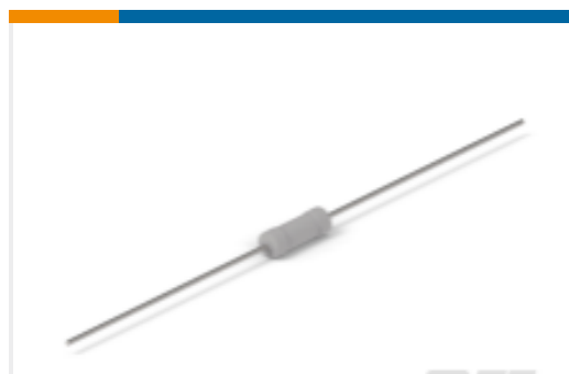
TE Part #7-1676123-7 1/2W SM M/OX 5% 1K2
