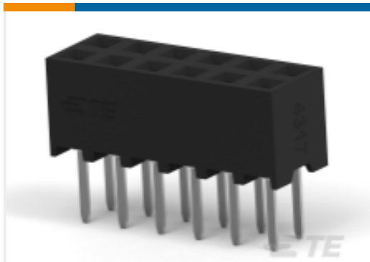
TE Part #1-2314821-4 14P,2MM,B-B,REC,DRVT,2.7,0.38AU,TB
