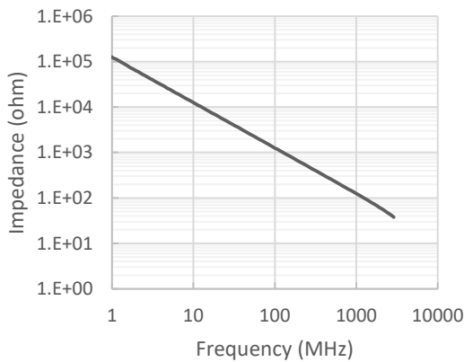
Impedance - Freq.
